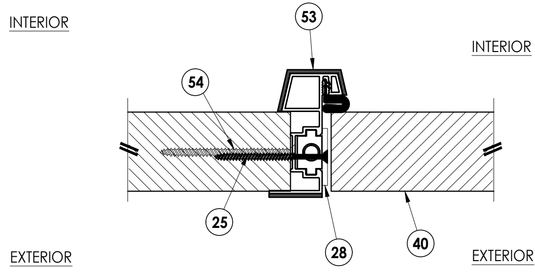
4 6 HORIZONTAL CROSS SECTION
