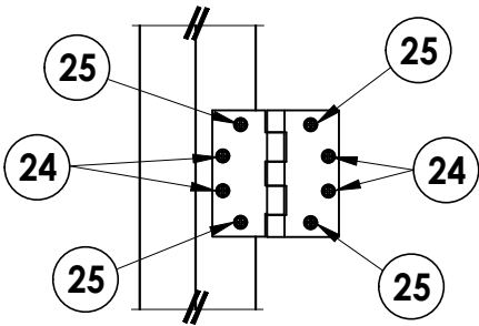
HINGE DETAIL
