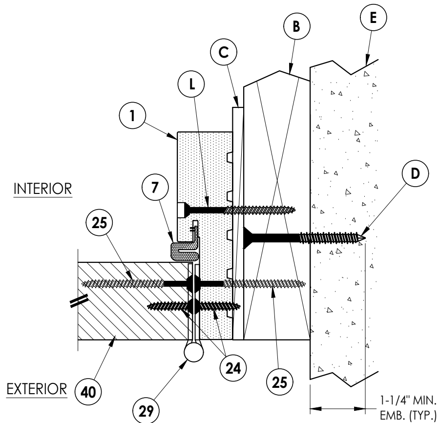
2 6 HORIZONTAL CROSS SECTION
