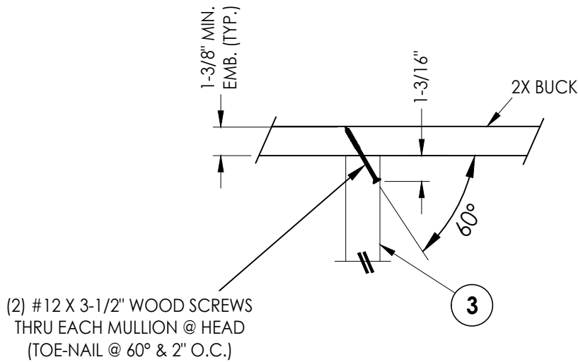
MULLION-TO-HEAD CONNECTION DETAIL
