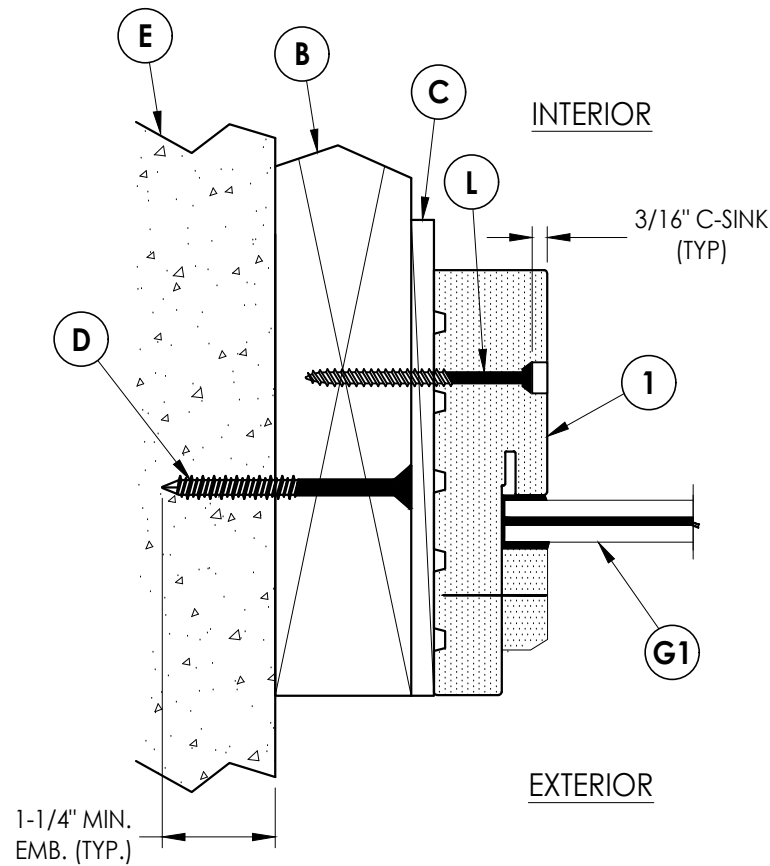
1 6 HORIZONTAL CROSS SECTION
