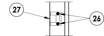
ROLLER LATCH STRIKE PLATE DETAIL
