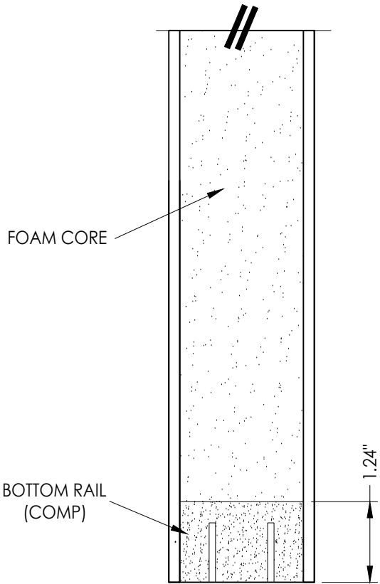
2 2 VERTICAL CROSS SECTION
